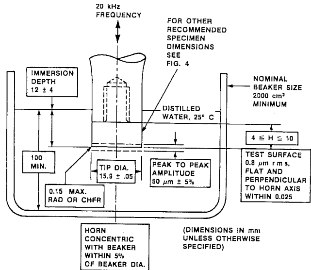
FIG. 1 Important Parameters of the Vibratory Cavitation Test
