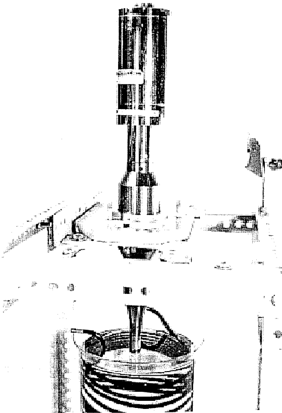
FIG. 3 Photograph of a Typical Apparatus
